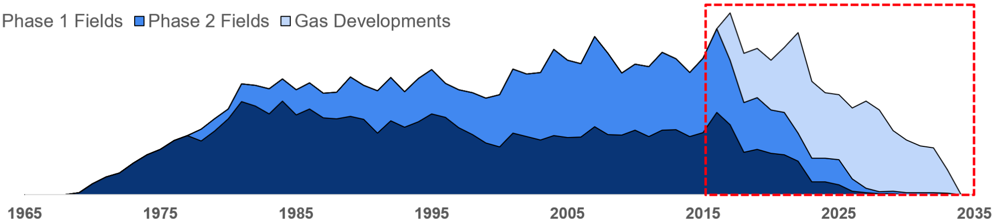
ANNUAL LONGFORD GAS PRODUCTION (PJ)
